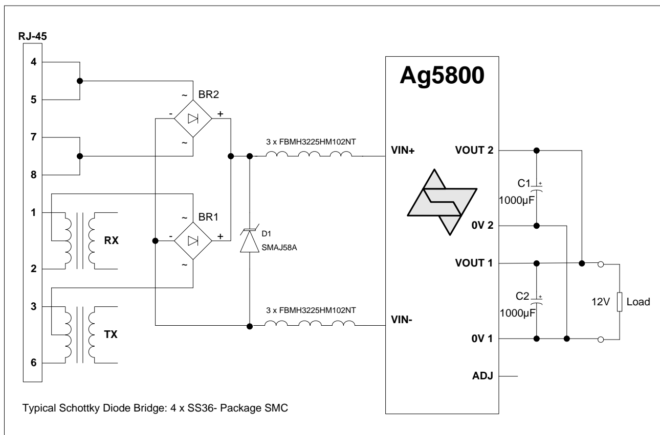
Figure 11: Typical Connection Diagram
