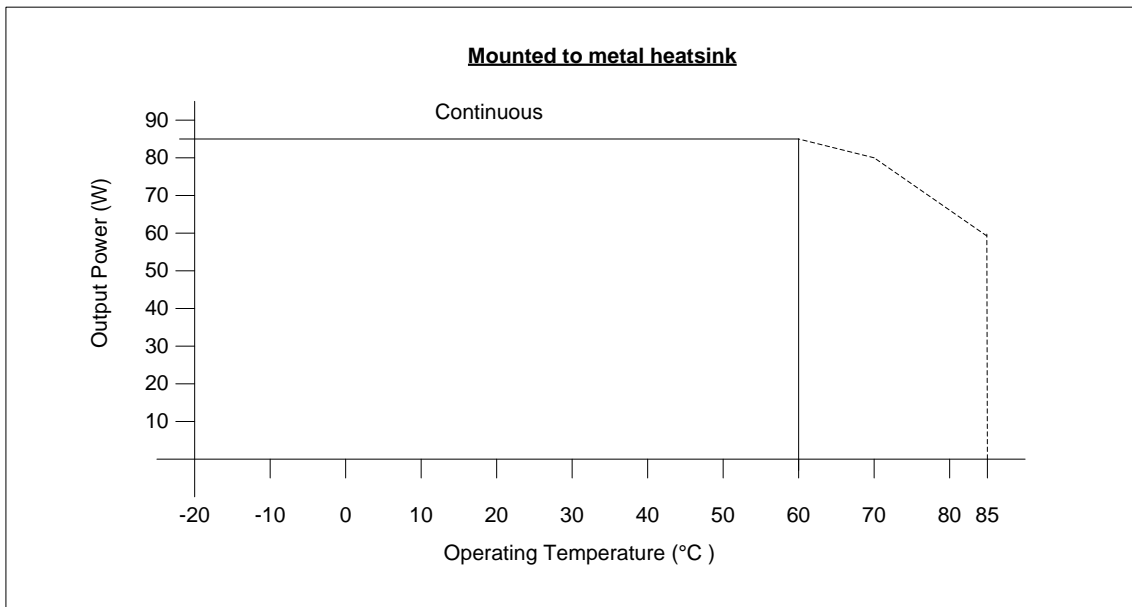
Figure 13: Operating Temperature (Thermally connected to PCB and enclosure)
