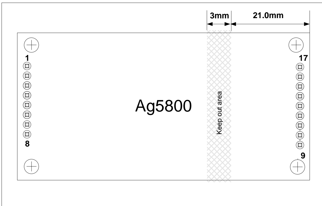
Figure 4: Position of the Isolation Barrier
