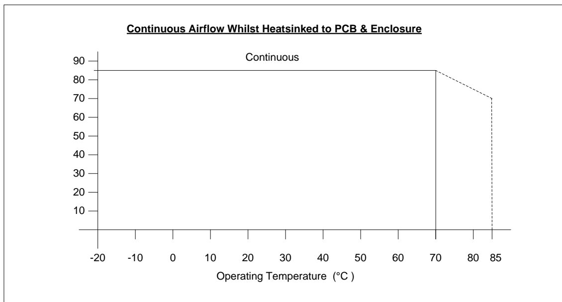
Figure 12: Operating Temperature
