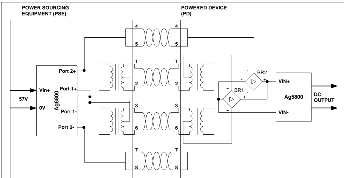
Figure 8a – Typical Application Diagram for Ag5800 using 10/100BASE-T
