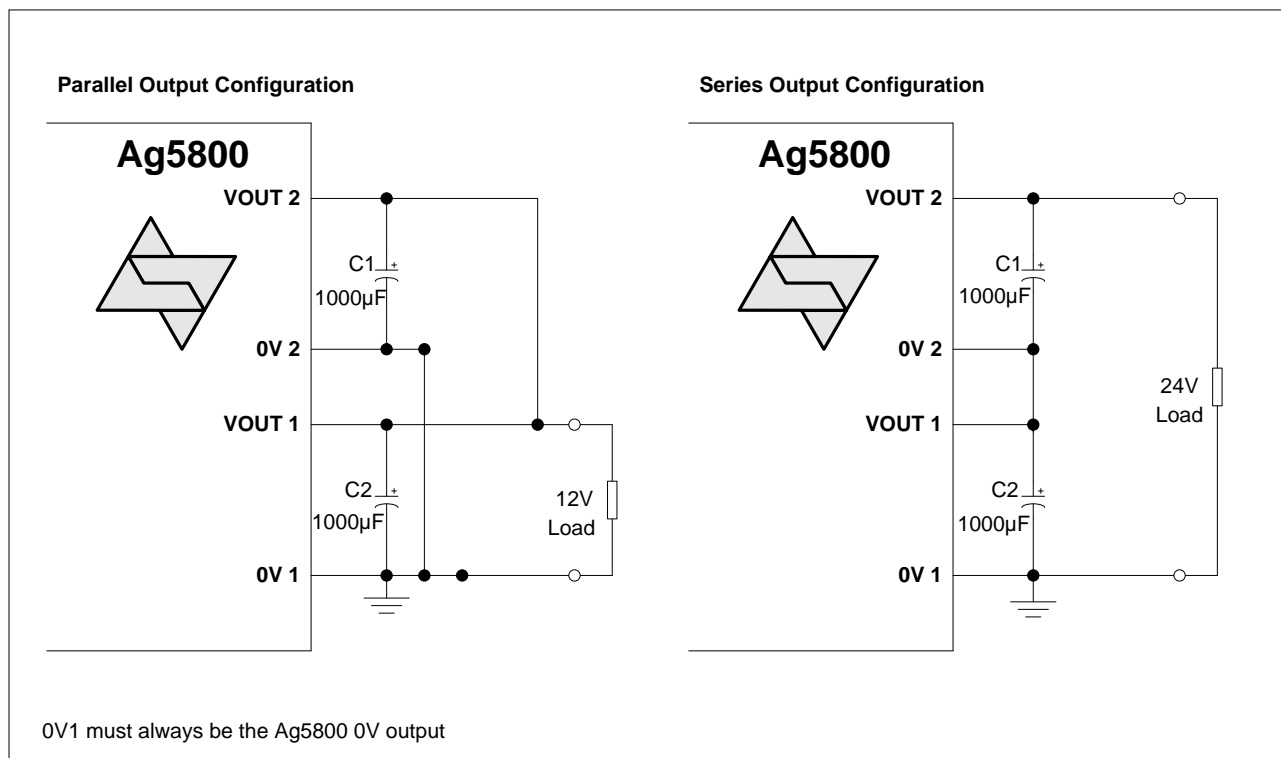
Figure 9: Output Configurations
