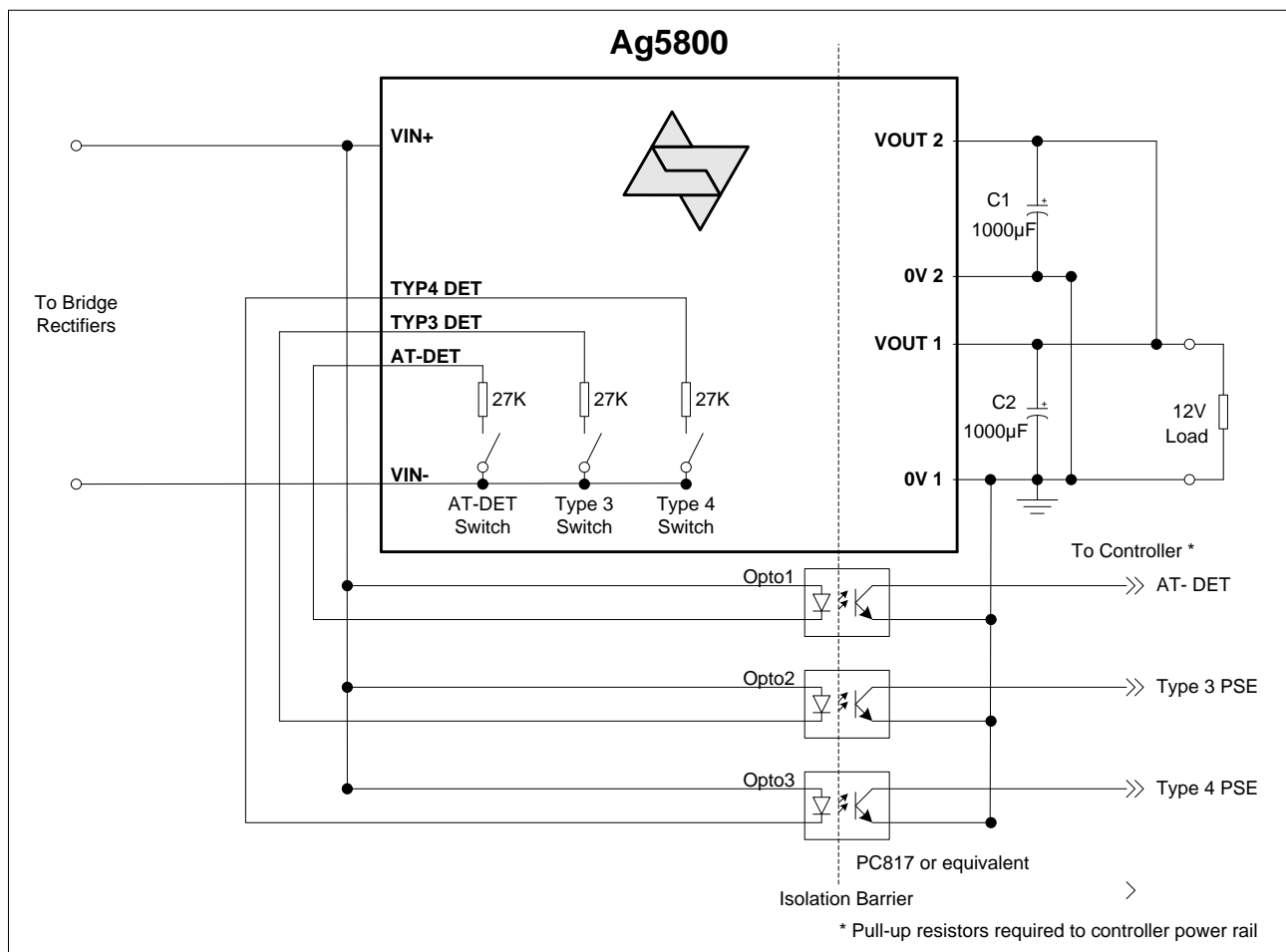
Figure 7: Physical Layer Detect Configuration
