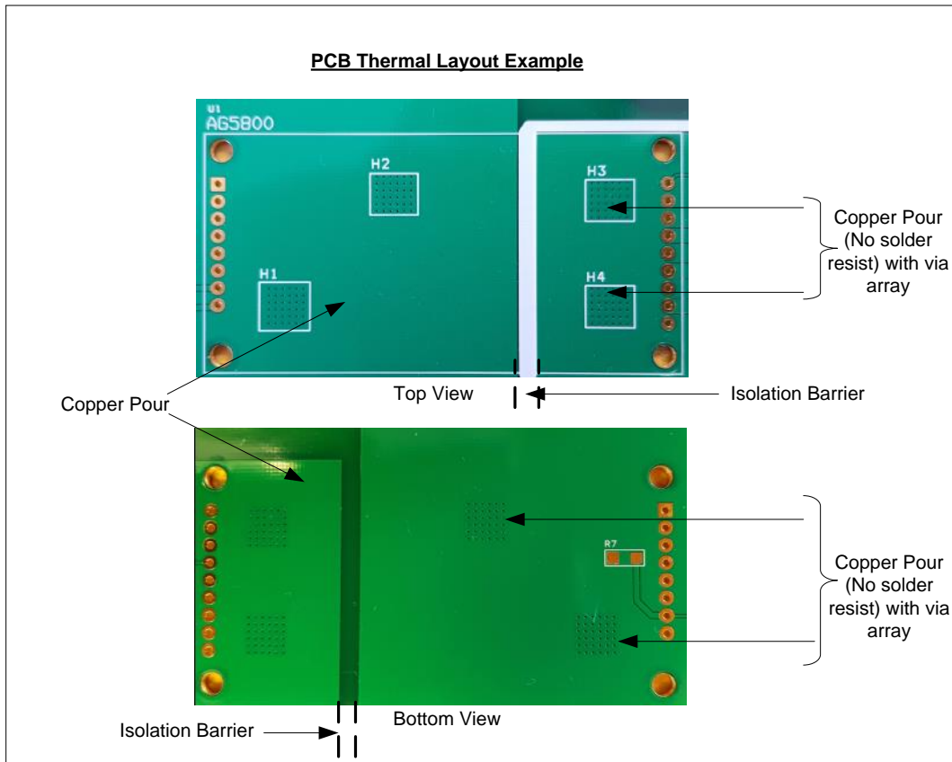
Figure 17: Suggested PCB Thermal Layout
