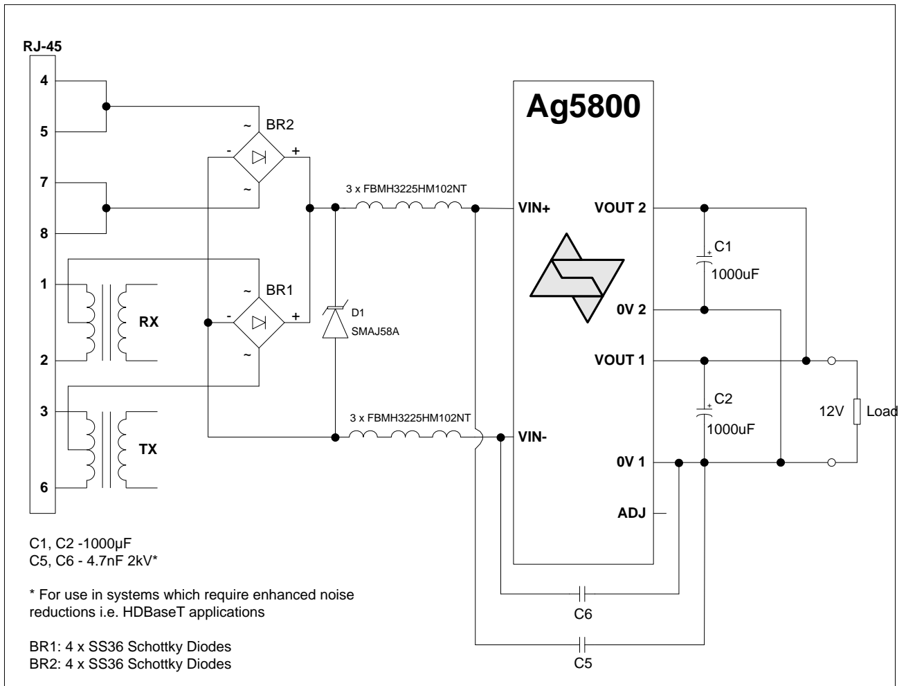
Figure 15: EMC Filtering
