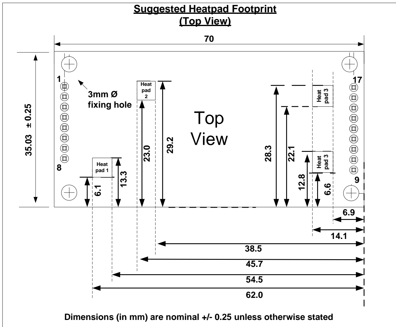
Figure 18: Suggested Heatpad Footprint
