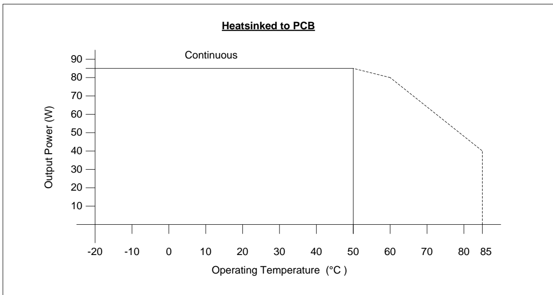
Figure 14: Operating Temperature (Thermally connected to PCB)
