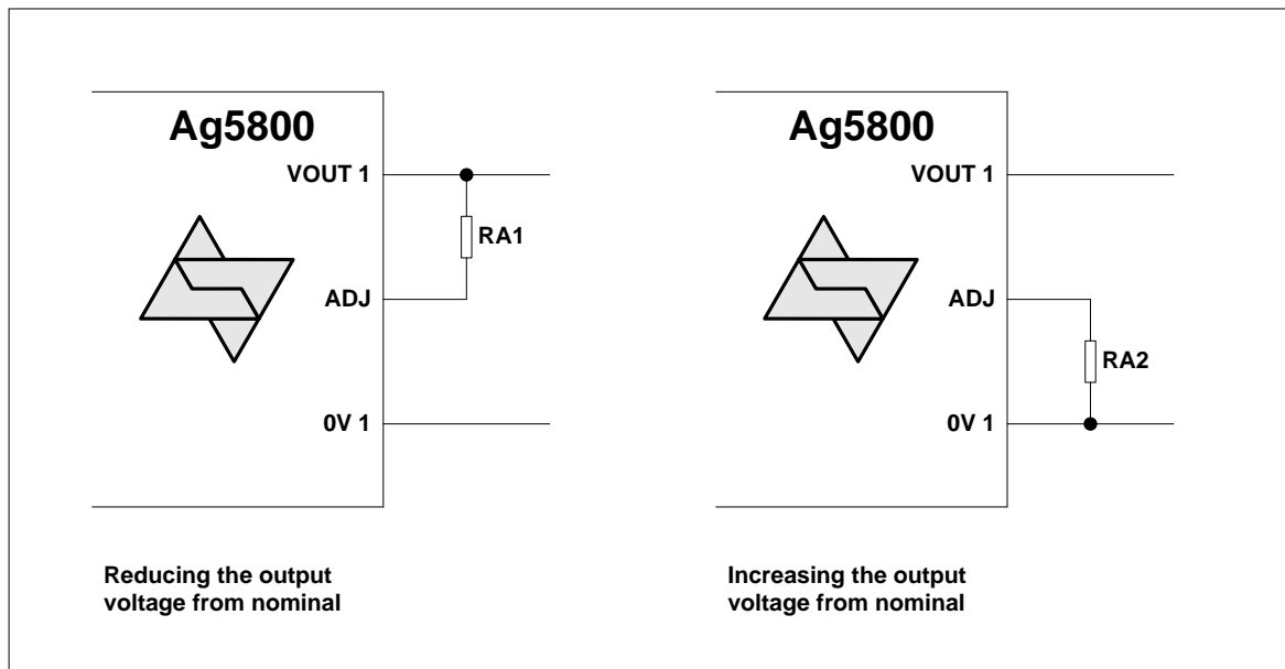
Figure 10: Output Adjustment
